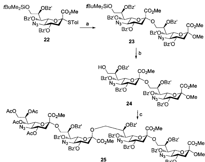
Scheme 4. a) 10 , NIS, TfOH, CH 3 CN, 3 Å MS, –40 °C, 1 h, 51 %, \alpha:\beta = 1.1:1 . b) HF/py, AcOH, THF, 1 h, 90 %. c) 21 , NIS, TfOH, CH 3 CN, 3 Å MS, –40 °C, 1 h, 32 %, \beta .
